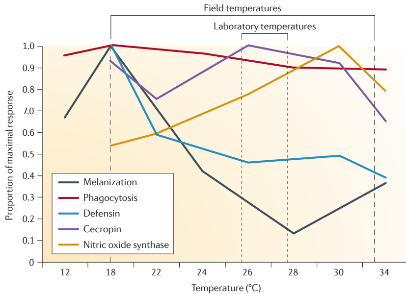
Figure 1 | Environmental temperature profoundly affects the rates of a range of humoral and cellular immune responses. Rates of immune and humoral responses are represented as the mean proportion of the maximal response. Melanization and phagocytosis were measured as the proportion of Sephadex beads that were fully melanized or the proportion of haemocytes that had engulfed fluorescent beads, respectively, in mosquitoes housed at different constant temperatures. Expression levels (cDNA counts) of genes encoding two antimicrobial peptides, defensin and cecropin, and nitric oxide synthase are also shown for mosquitoes housed at different constant temperatures. These results clearly indicate that the immune phenotype described under laboratory conditions (26–28 °C) is not the same as the phenotype expressed across the range of possible field temperatures for parasite transmission (18–34 °C), and current laboratory studies on mosquito innate immune functions are missing potentially important biological complexity. Figure is modified from REF. 44.
