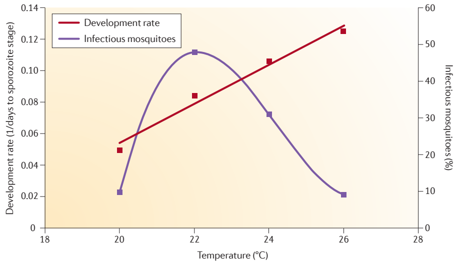
Figure 2 | Changes in ambient temperature differentially affect two parasite traits. The proportion of infectious mosquitoes (that is, the proportion with sporozoites in their salivary glands) can be used as a measurement of parasite survival, and parasite development rate is measured as the reciprocal of the number of days taken to reach the sporozoite stage. Although parasites develop to the sporozoite stage at faster rates with increasing ambient temperature, the proportion of infectious mosquitoes sharply declines as the ambient temperature rises above 22 °C. The data shown are for Plasmodium yoelii infecting Anopheles stephensi . Figure is modified from REF. 53.
